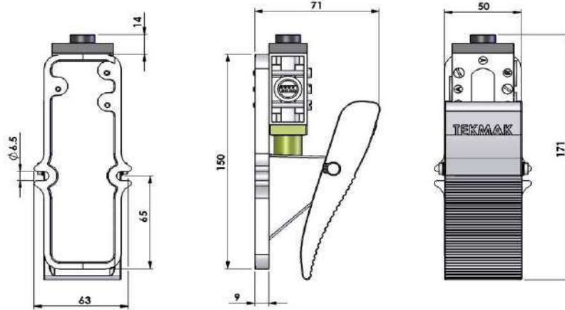
TAY-32 Normalde Kapalı Normally Closed
