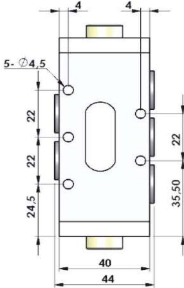
TPP-52 Normalde Kapalı Normally closed
